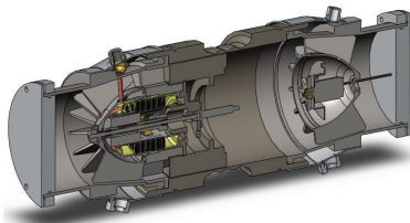
Cutaway of Fuel Flow Transmitter
